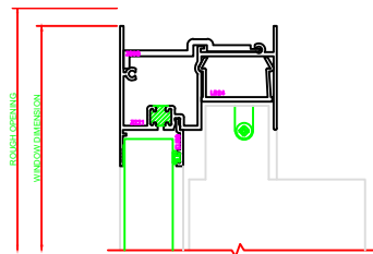
101 HEAD SERIES: 3500
